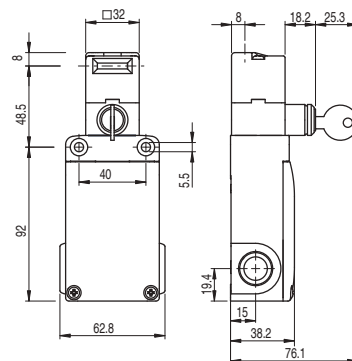
Switch FS ●●98D●●● Operating principle D with auxiliary key release
