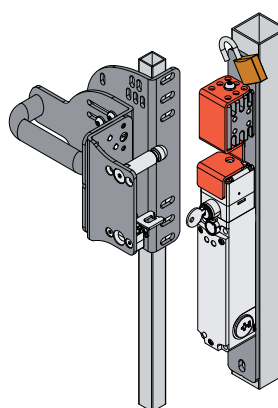
Lock out device closed. Padlock insertion.
